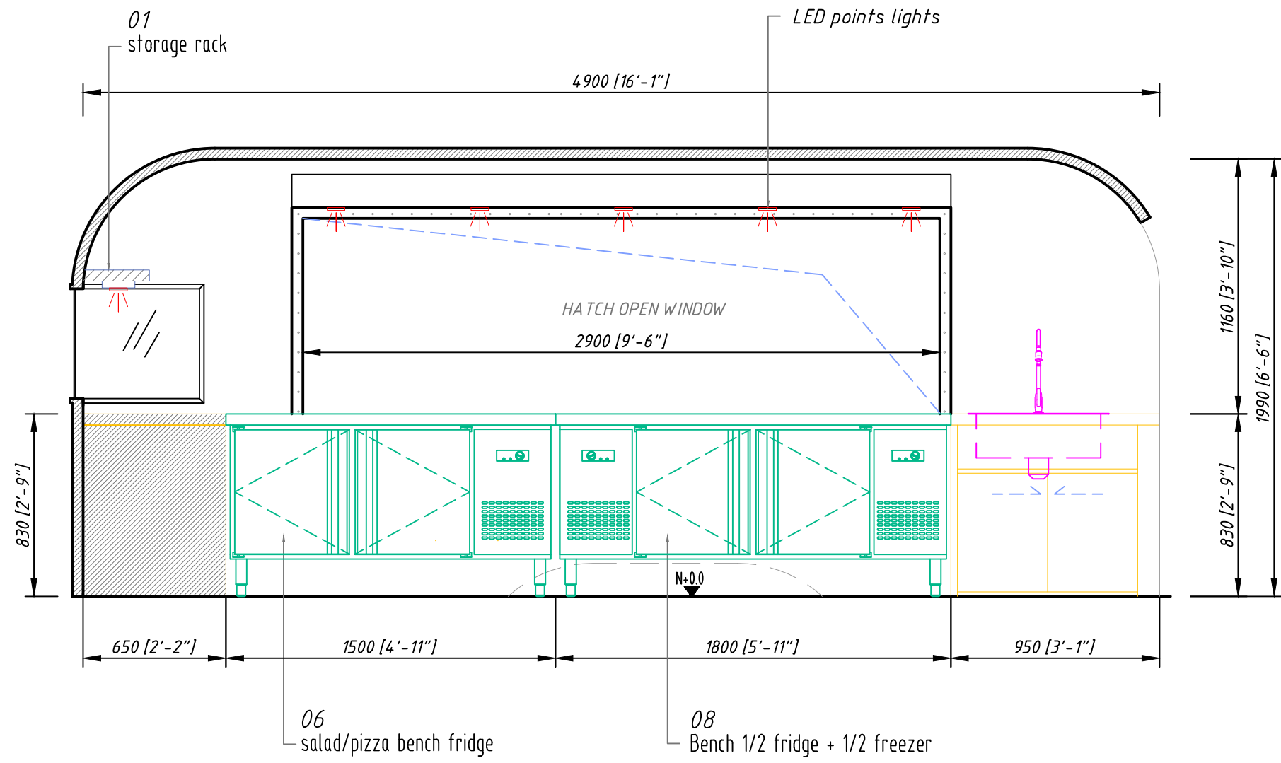
FOOD TRUCK SECTION_2-2
