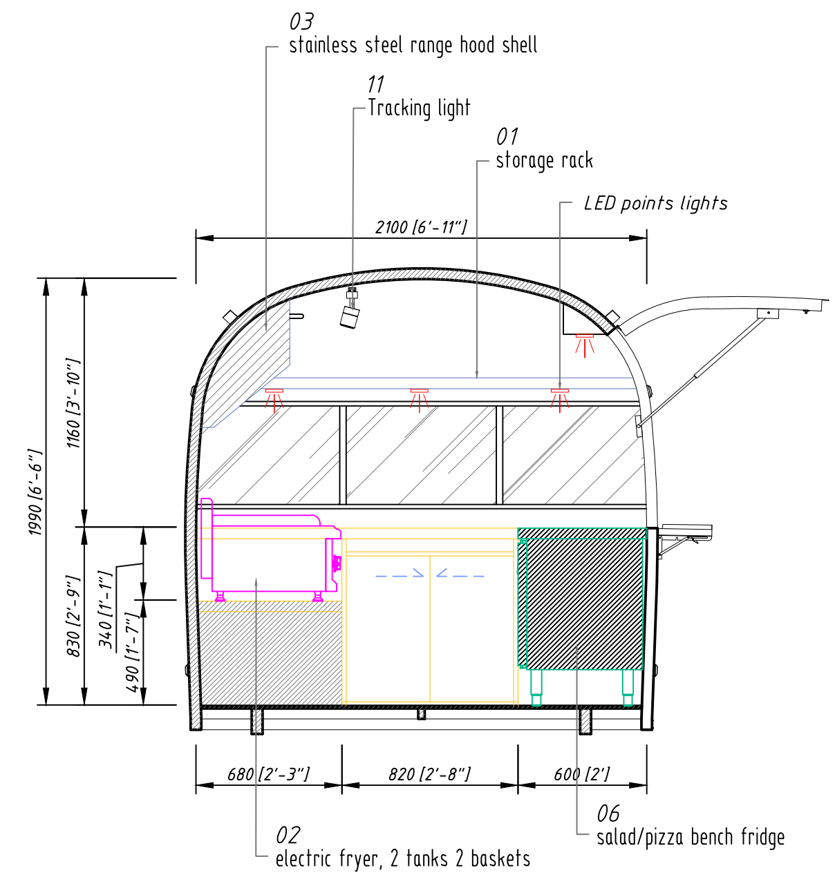
FOOD TRUCK SECTION_3-3
