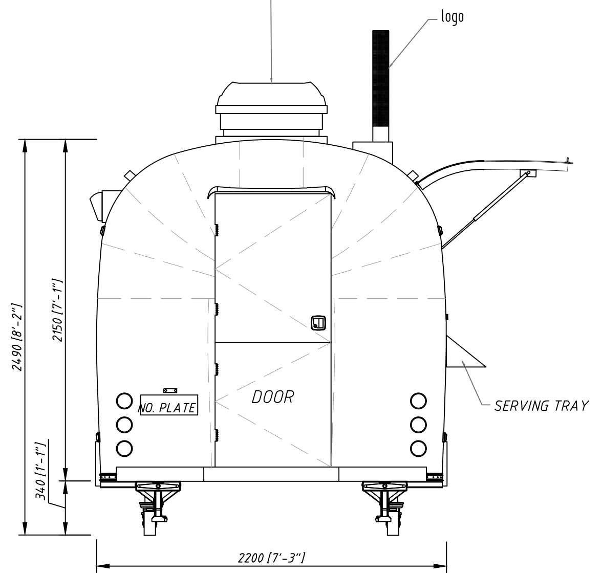
FOOD TRUCK CUSTOM SIDE ELEVATION_D
