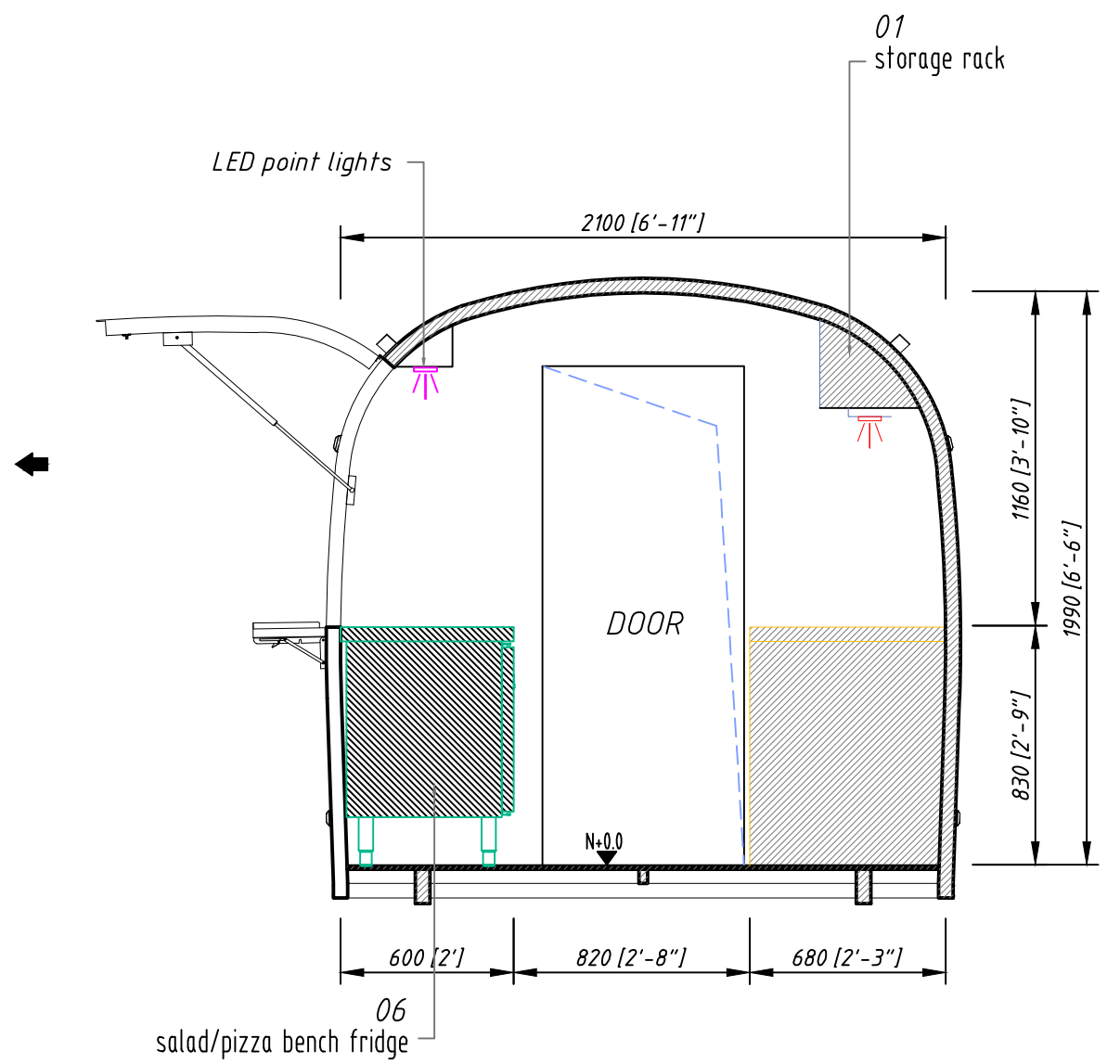
FOOD TRUCK SECTION_4-4
