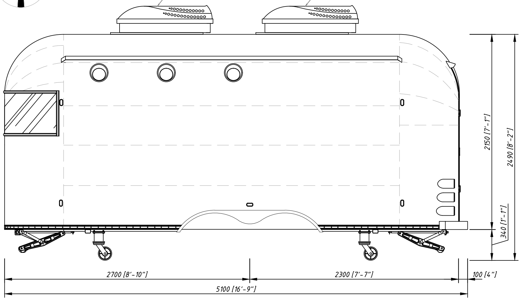
FOOD TRUCK CUSTOM SIDE ELEVATION_A
