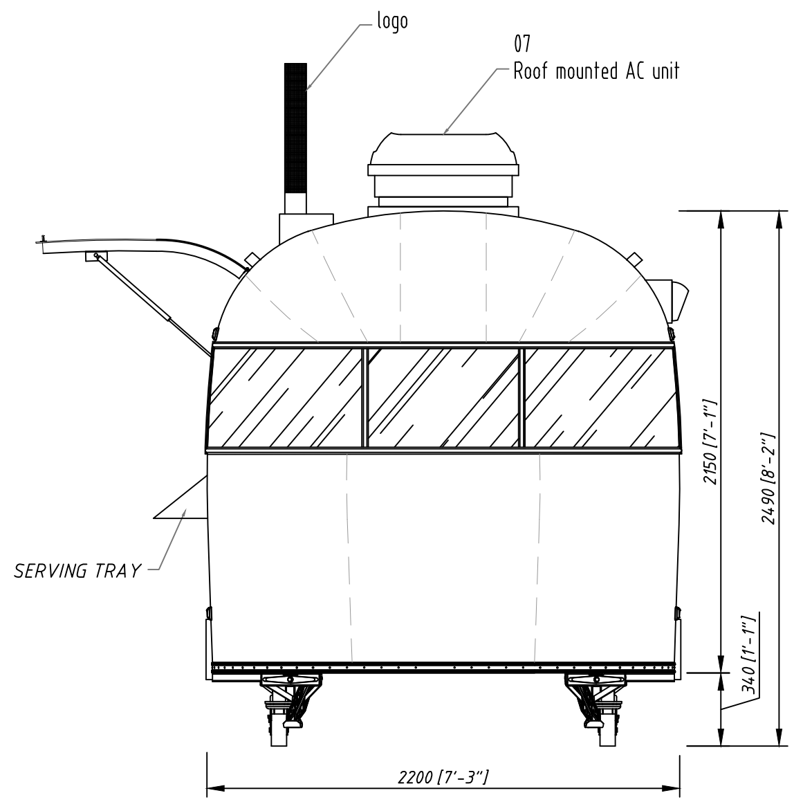
FOOD TRUCK CUSTOM SIDE ELEVATION_B
