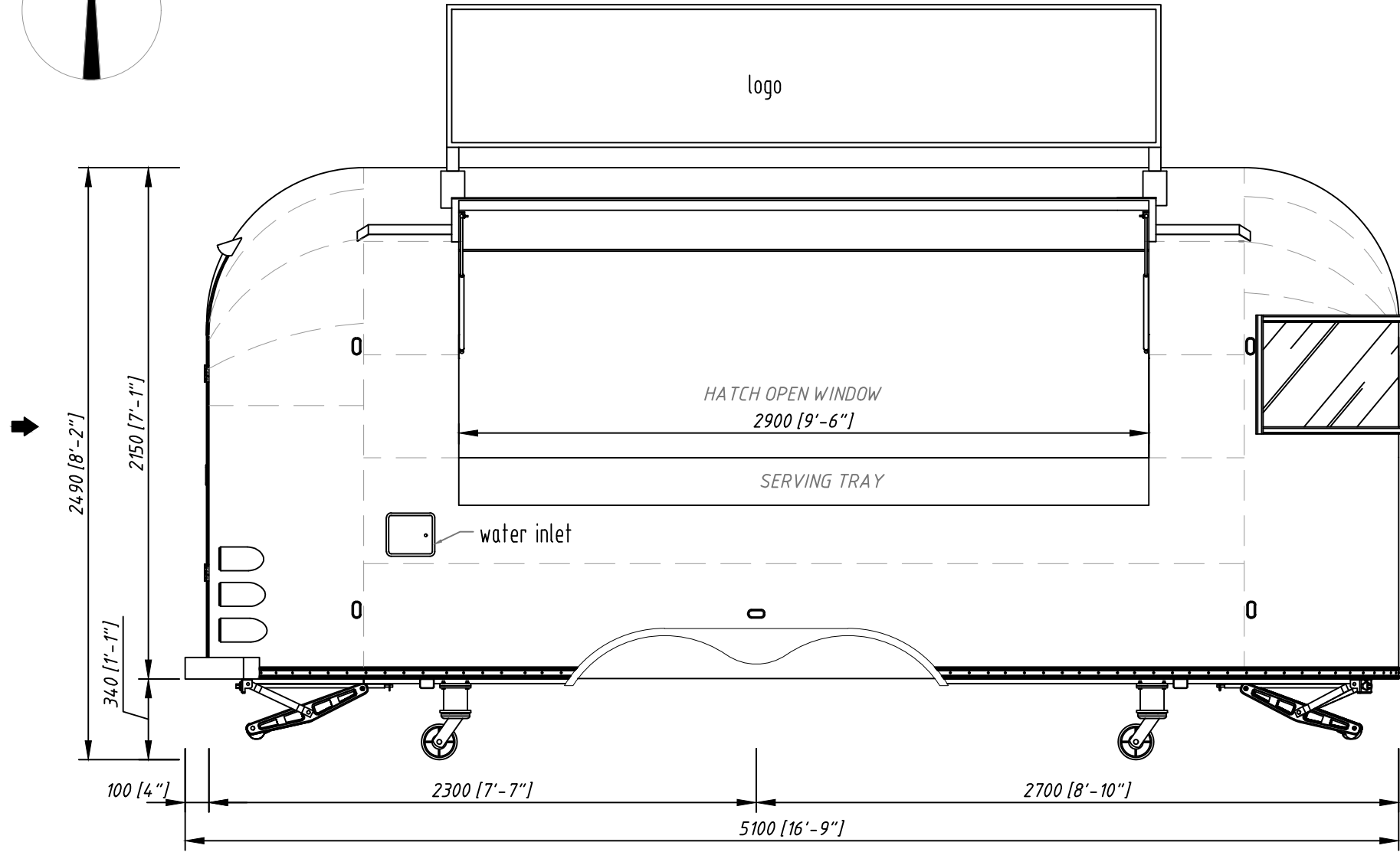
FOOD TRUCK CUSTOM SIDE ELEVATION_B
